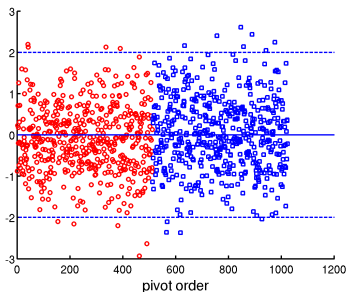
(b) Simulated Annealing
